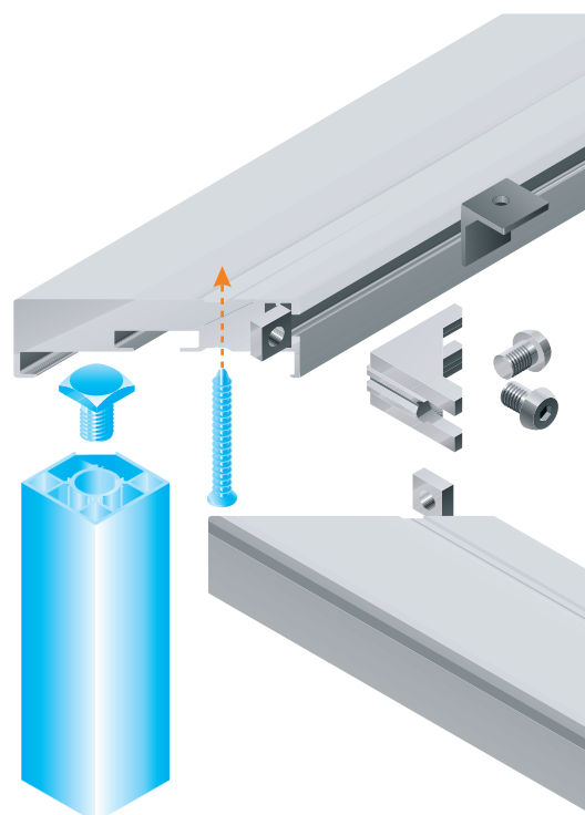
PMO.PS1 picior aluminiu, 40x 40mm
